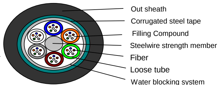
44~72 Core
