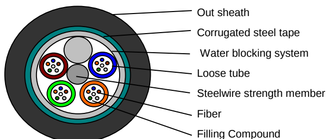
2~42 Core
